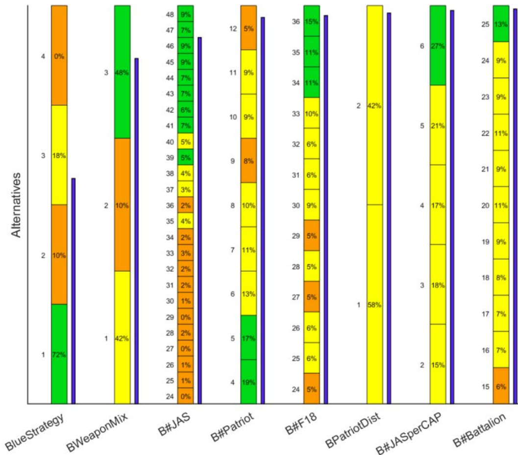
Figure 9: Skewed distribution analysis.
